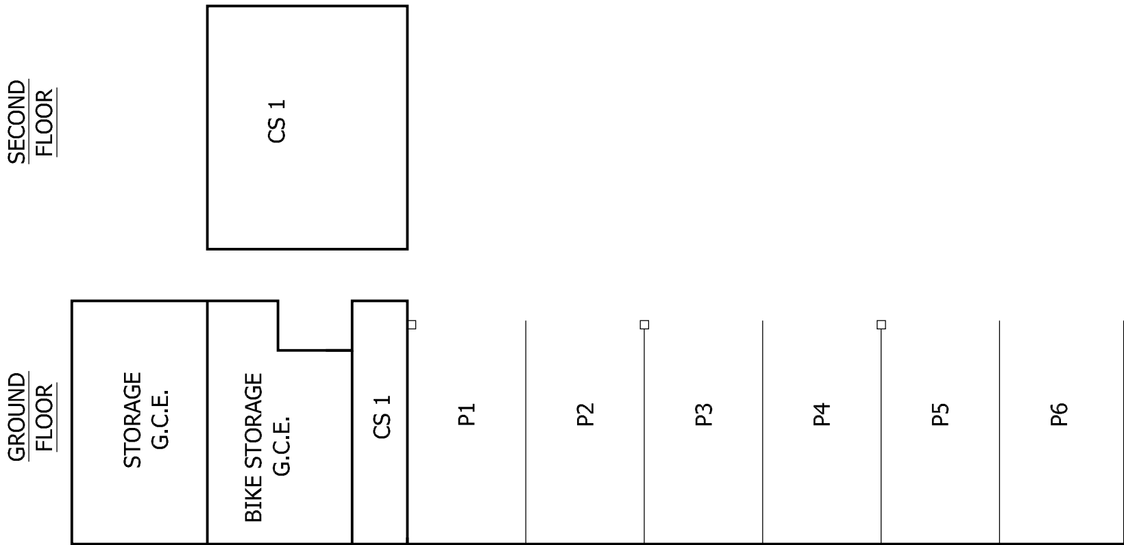
3 BUILDING 1 PLAN 1" = 10'-0"
